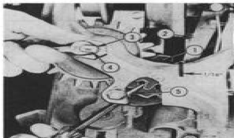
Fig. 27 — TWINE HOLDER DISC ADJUSTMENT
