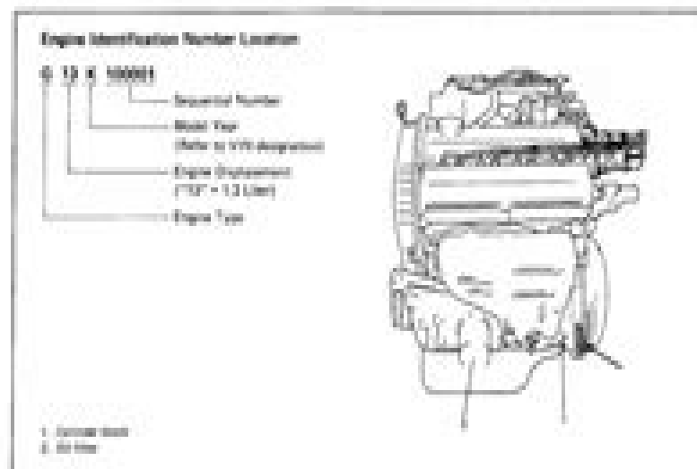
Fig. 54-3 Engine Identification Number Location
