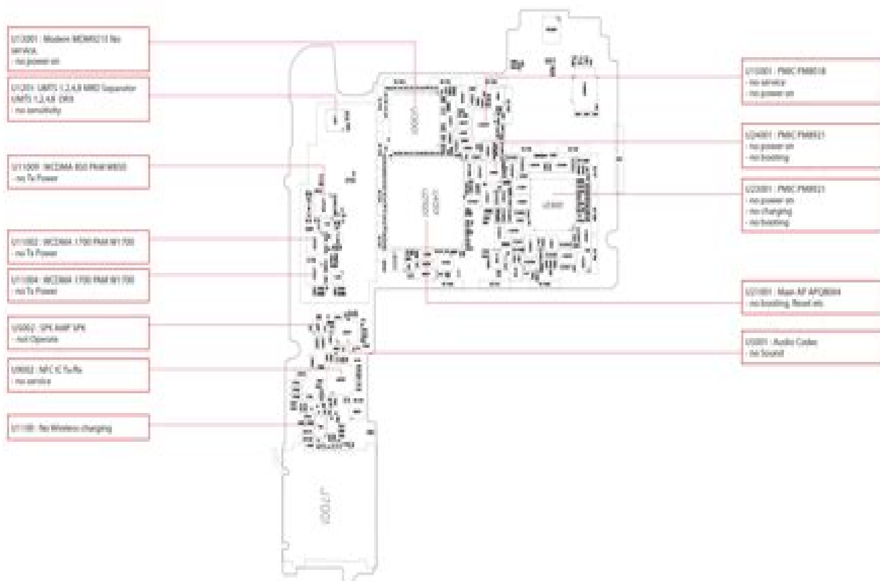
LG-E960_MAIN_EAX65044001_1.0_TOP
