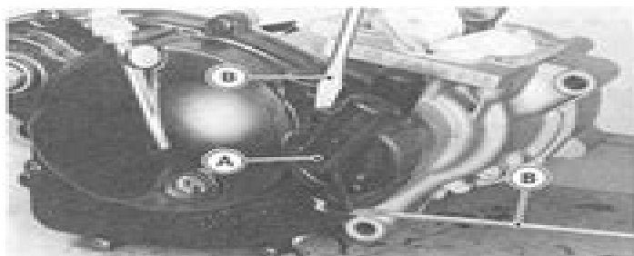
A. Water Pump Cover B. Screwdriver
