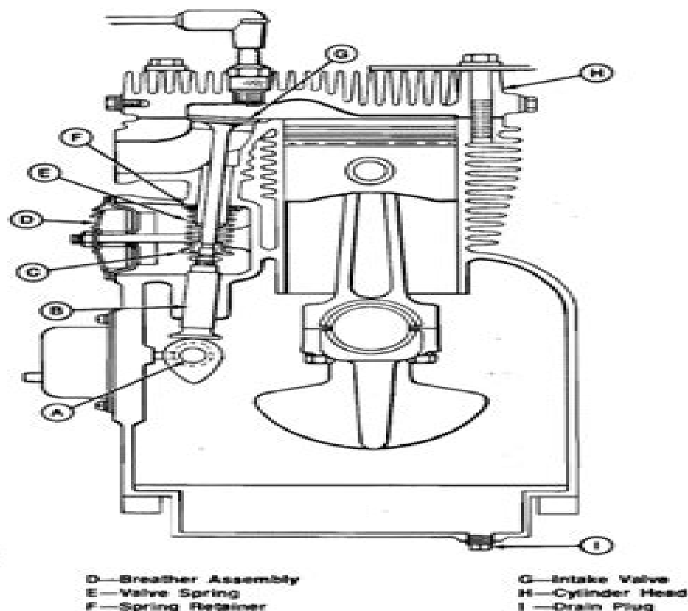
Fig. 1—Schematic View of Cylinder Head, Valves and Breather
