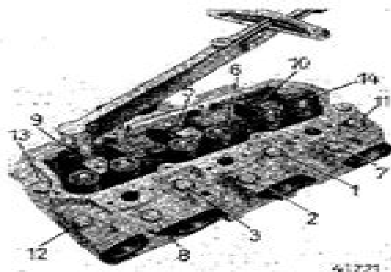
Fig. 6 - Correct Sequence for Tightening Cylinder Head Cap Screws
