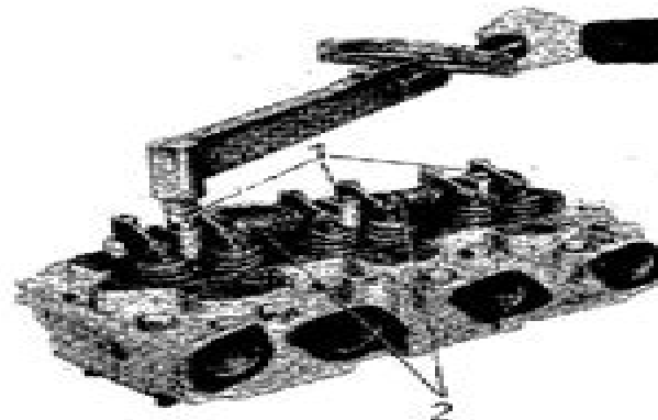
Fig. 7 - Tightening Rocker Arm Shaft Assembly 1 Cap screws 2 Rocker arm shaft assembly
