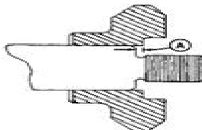
Fig. 6—Adjusting Row Unit Drive
