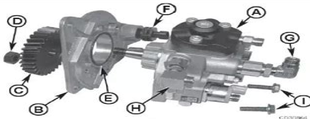
High pressure fuel pump exploded view
