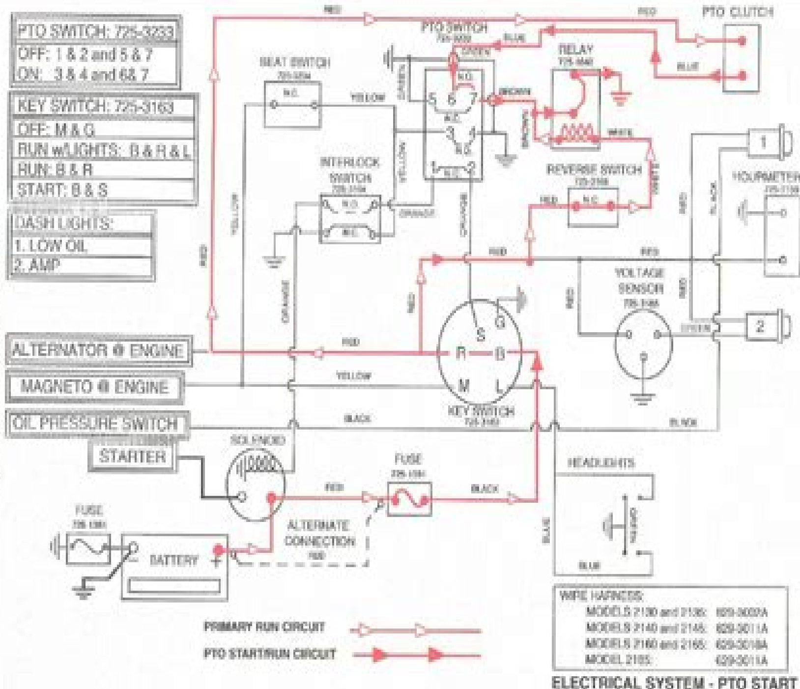
Figure D-8. PTO Startrun, All Models. D-12
