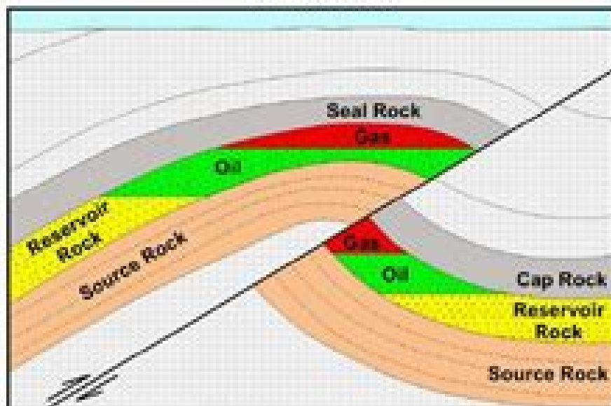
Thrust Fault
