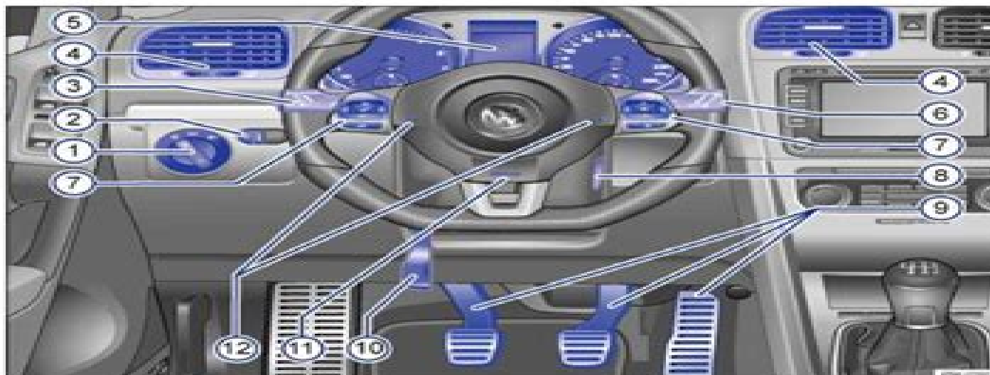
Fig. 5 Driver side-overview.
