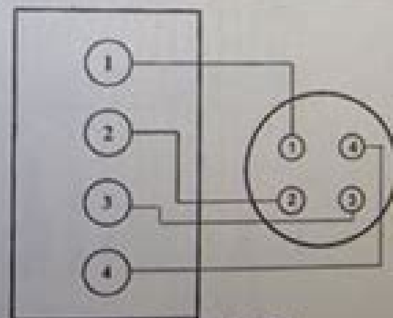
Fig. 272 Firing order diagram - certain 3.0L engines with EST ignition systems, please confirm with the firing order stamping on your engine and the cap-to-plug wire routing
