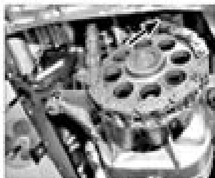
12.4 Pump against the chain tensioner
