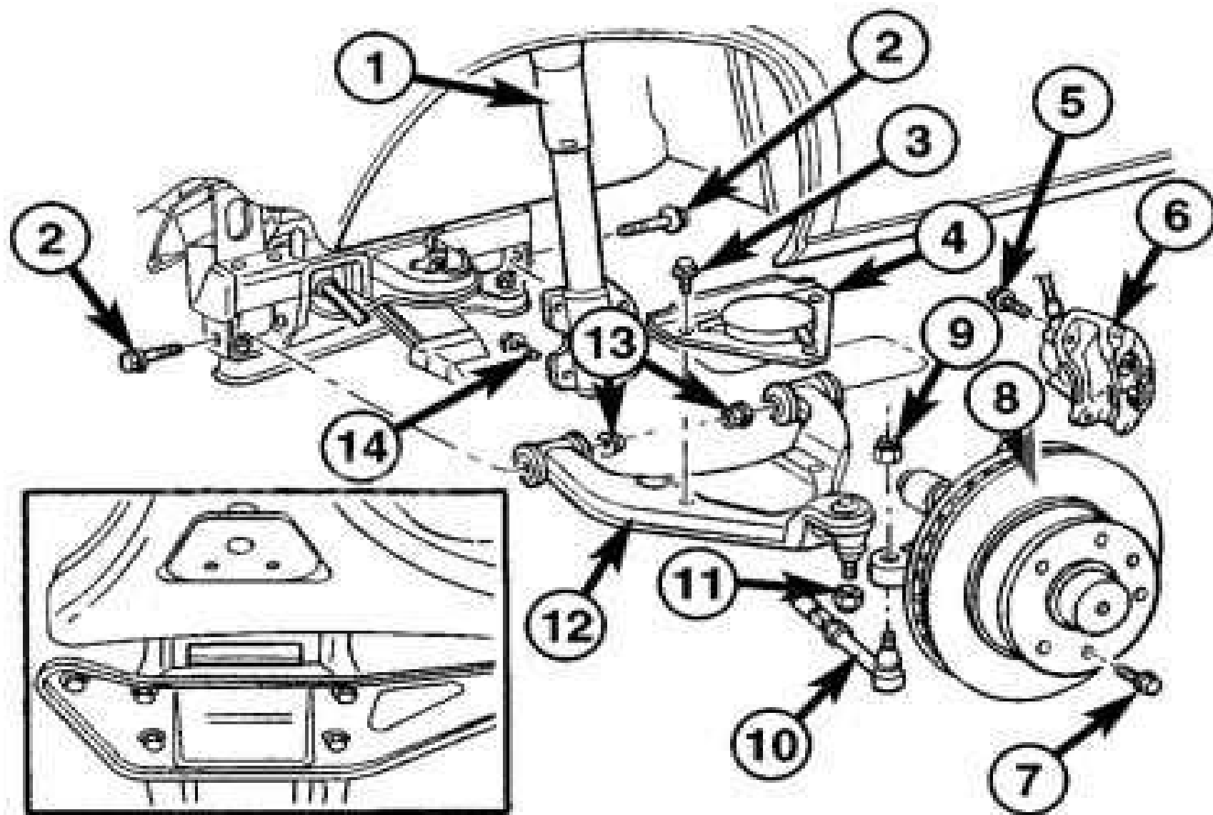
Fig. 8 LOWER CONTROL ARM
