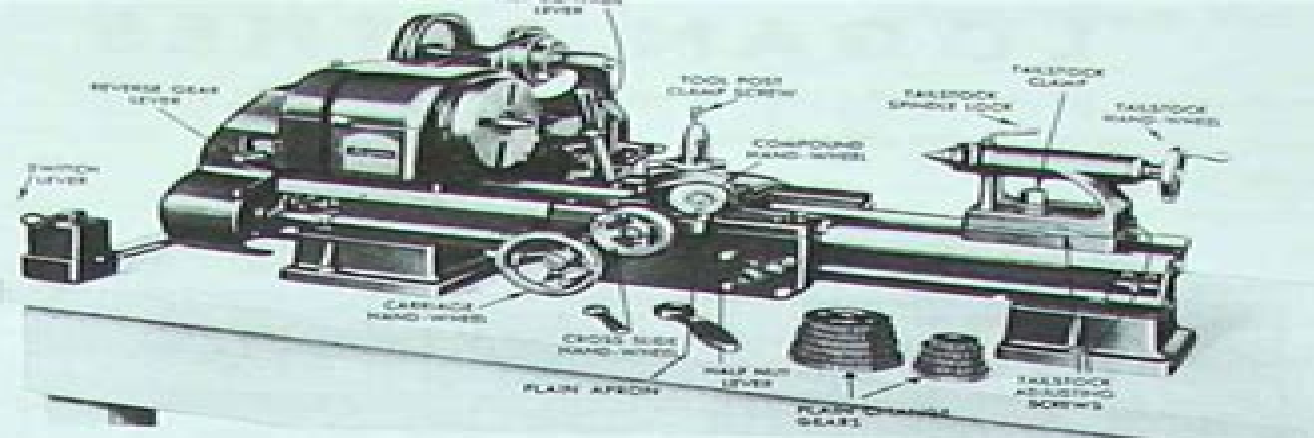
FIGURE 1—No. 9828-41 OR 9817-41 PLAIN CHANGE, PLAIN APRON 17" AND 28" CENTERS
