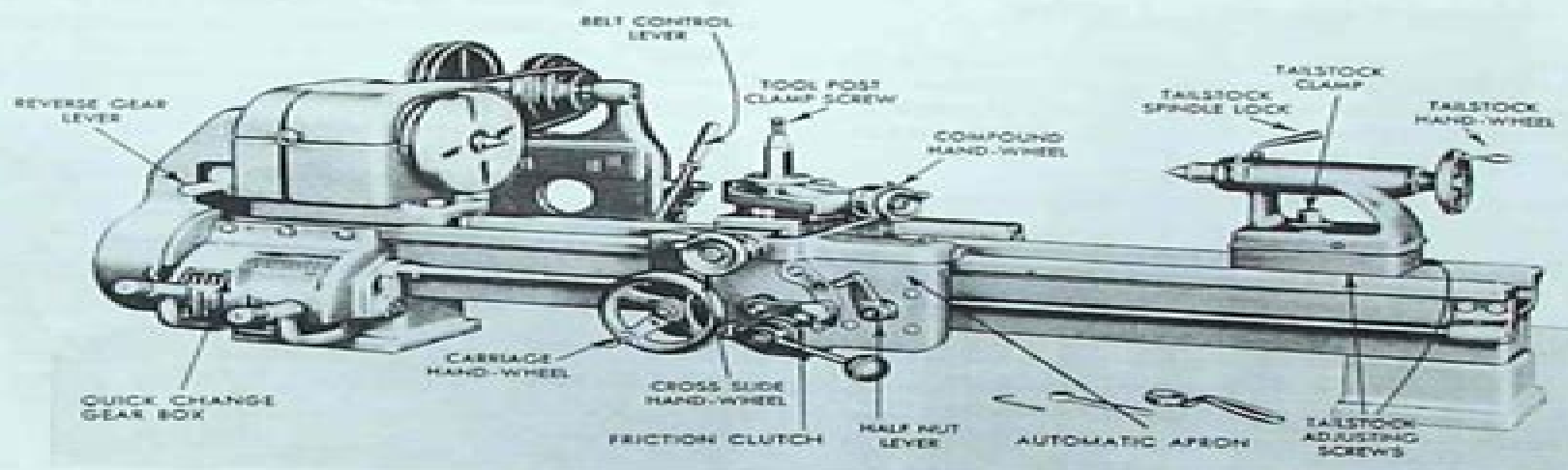
FIGURE 2—No. 9828-1 OR 9817-1 QUICK CHANGE GEARS, AUTOMATIC APRON 17" AND 28" CENTERS
