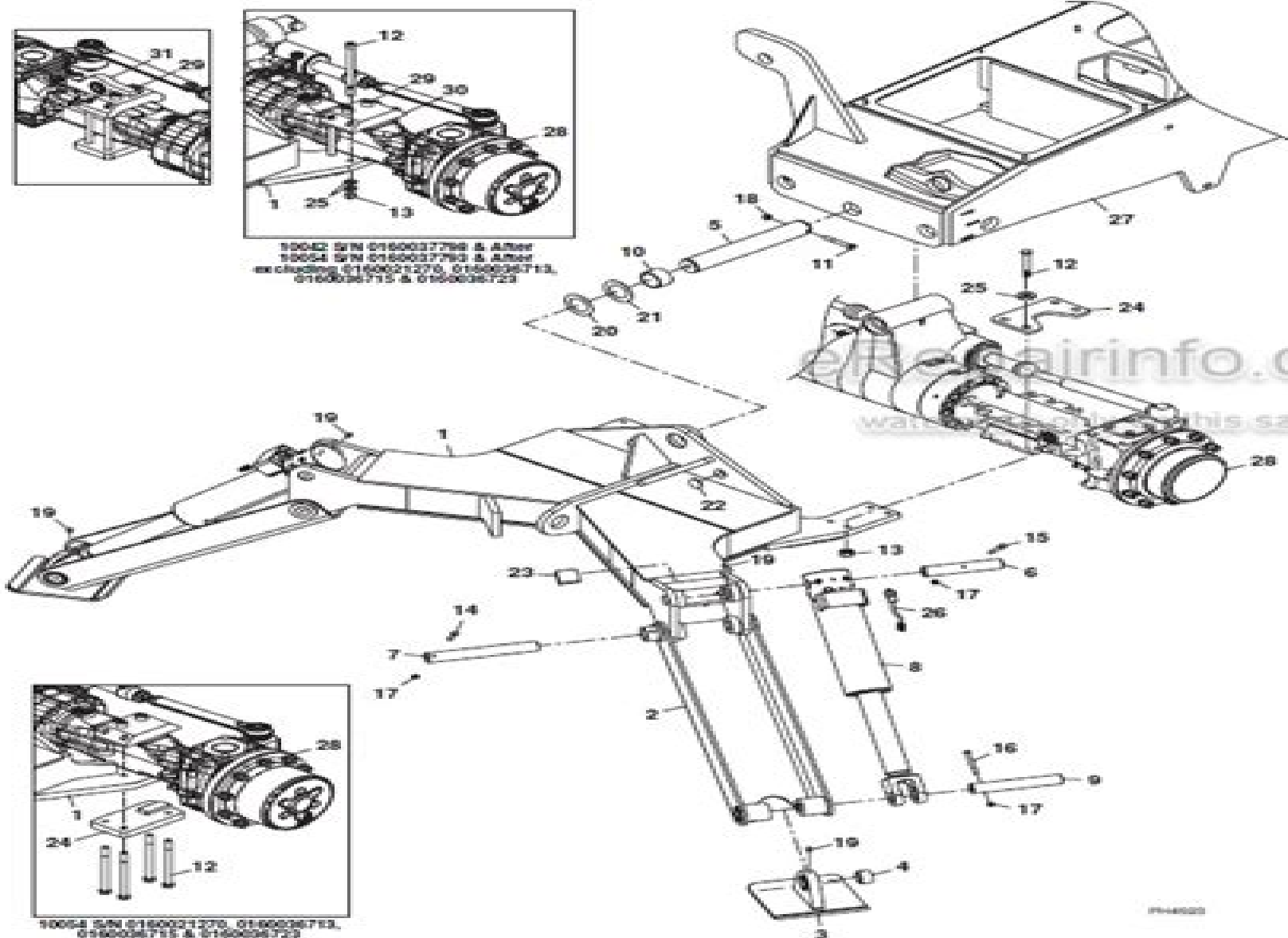
Figure 1-3 Outrigger Mounting
