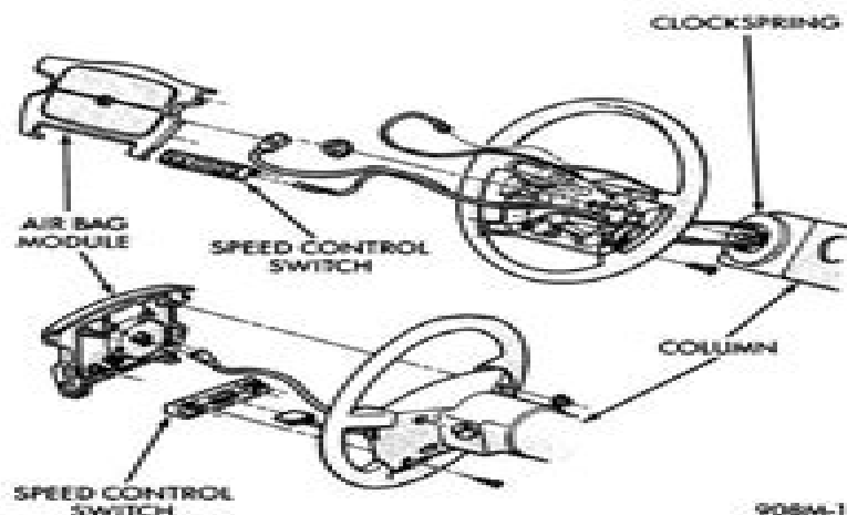
Fig. 6 Speed Control Switch Remove/Install
