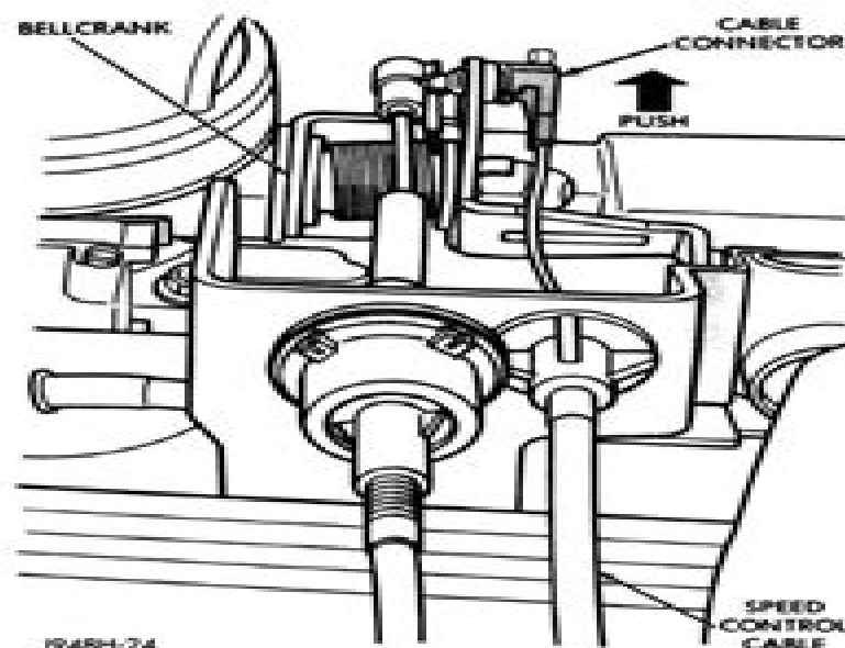
Fig. 7 Servo Cable to Bellcrank—Remove/Install
