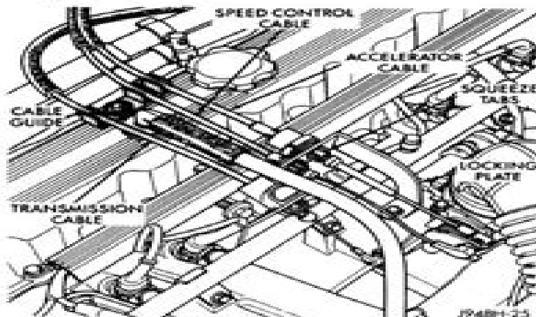
Fig. 8 Servo Cable to Locking Plate—Remove/Install
