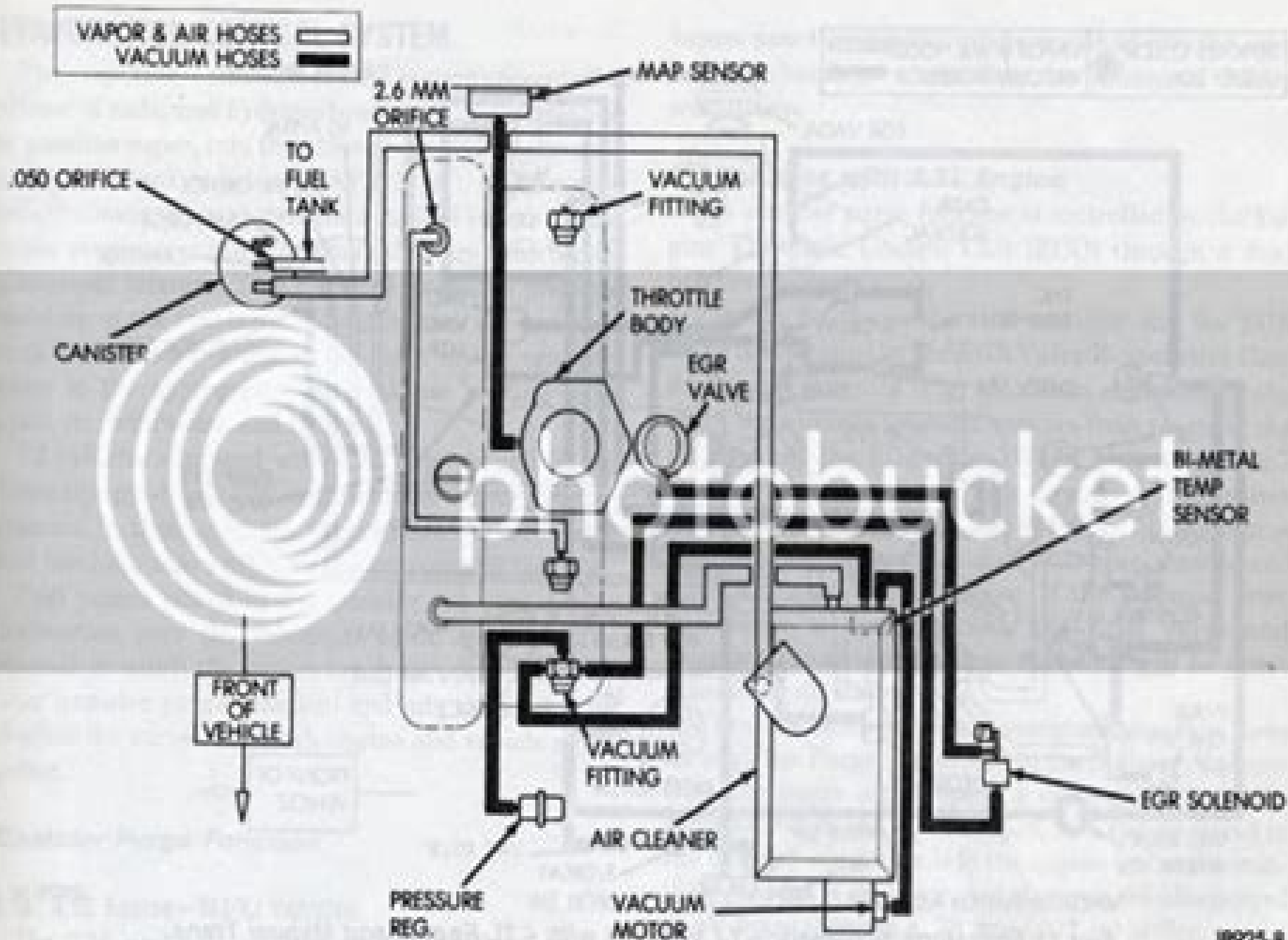
Fig. 9 Emissions Schematic—4.0L Engine
