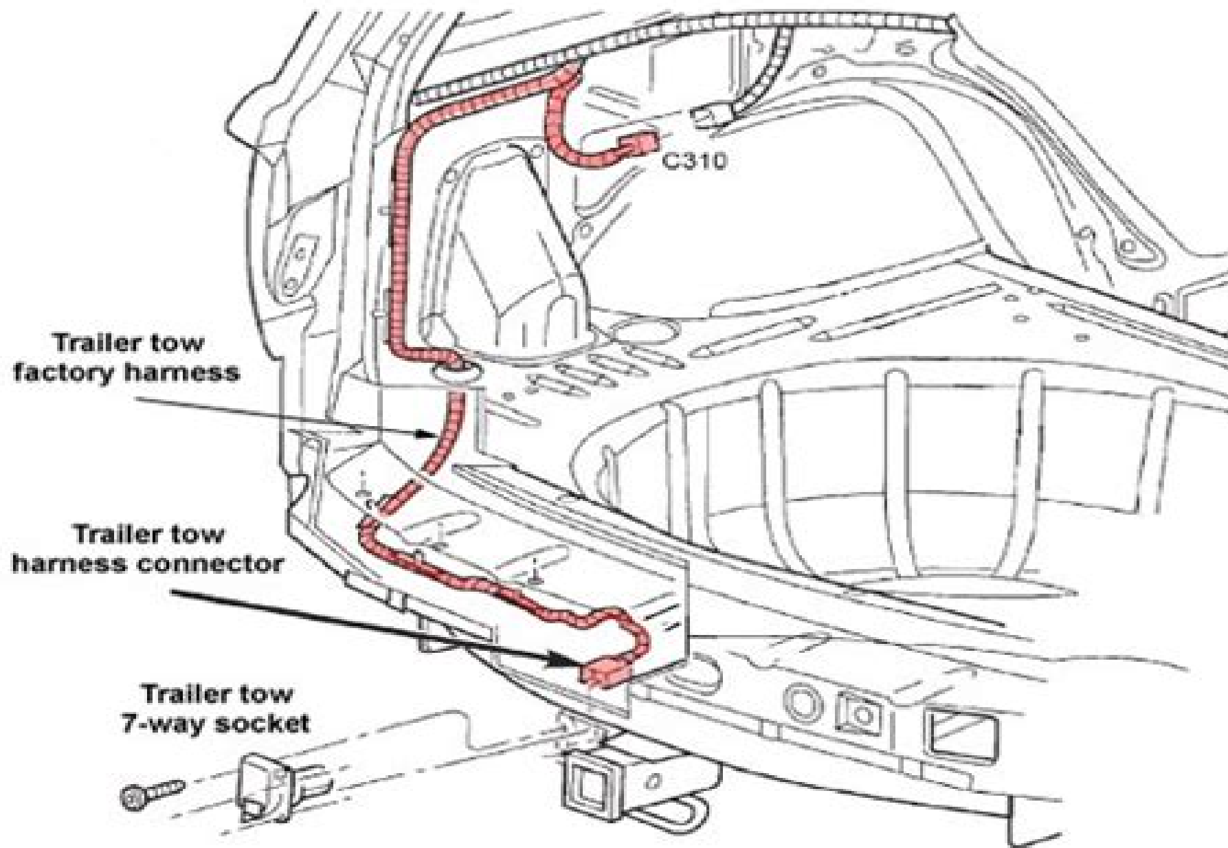
WJ left side cargo area - trailer tow factory harness routing
