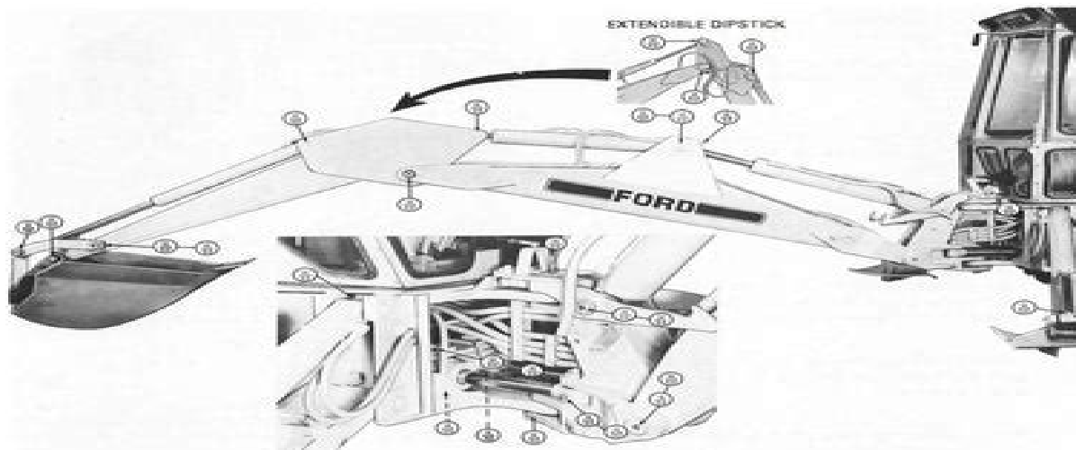
Figure 77 Backhoe Lubrication Fittings
