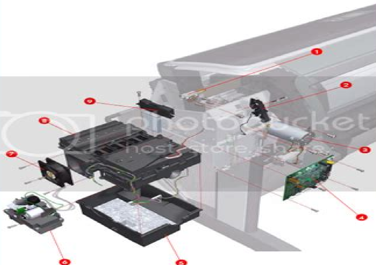
Figure 7-6: Right Hand Assemblies
