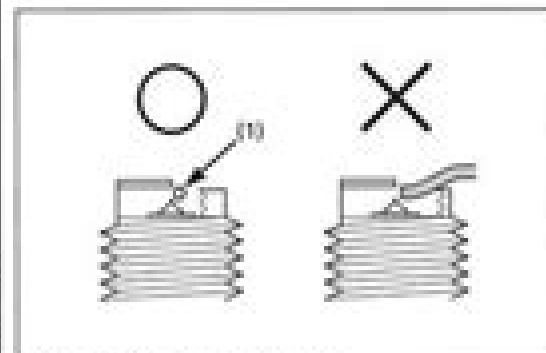
(1) WIRE TYPE FEELER GAUGE
