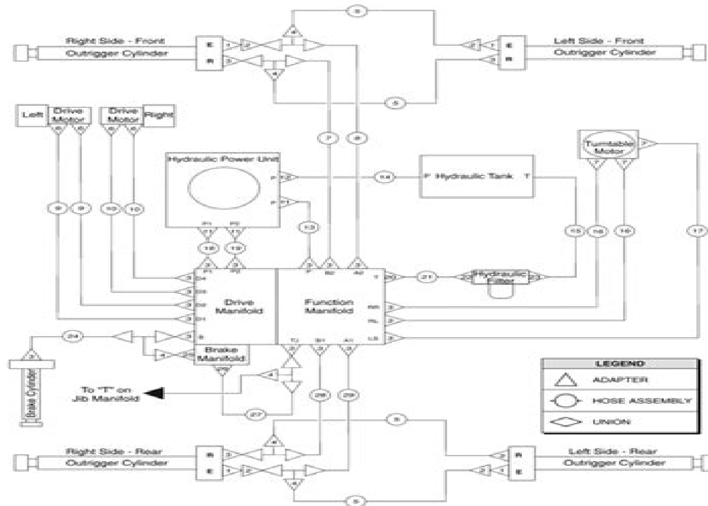
Figure 605.1 Rev B Description Hydraulic Hoses and Fittings - Chassis
