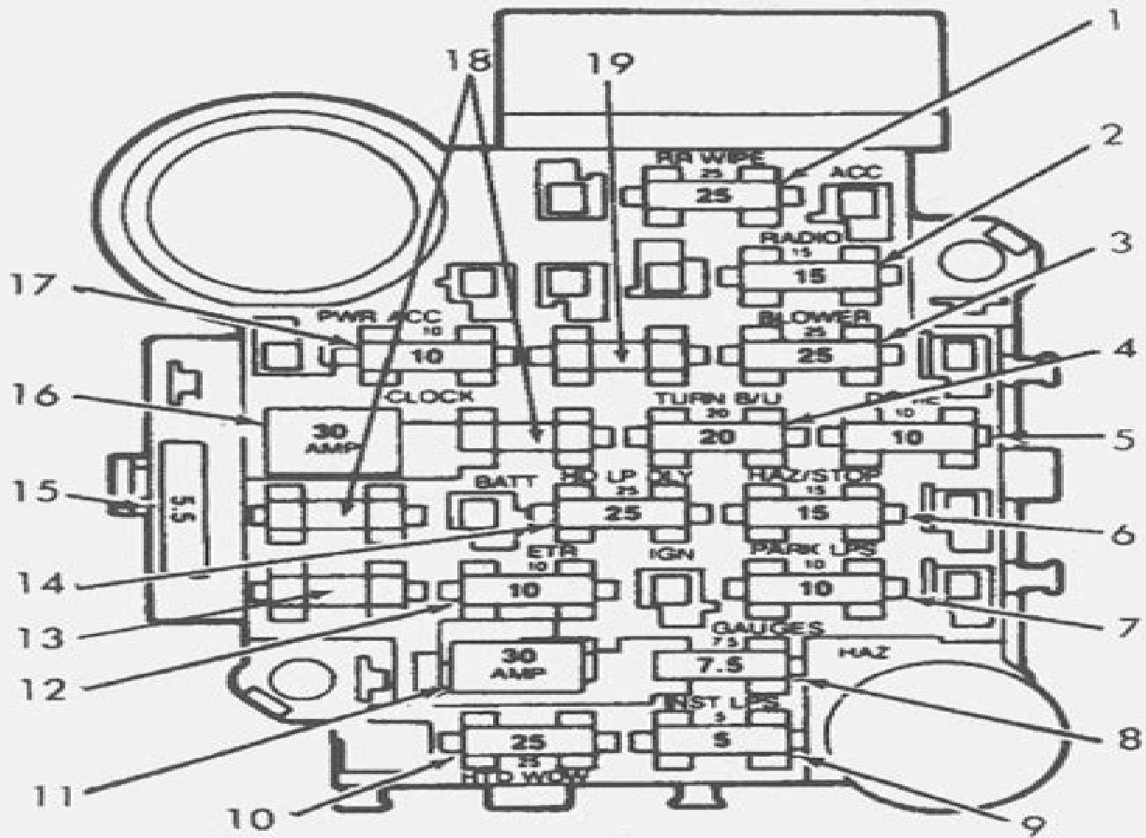
1984 - 1988 AMC style fuse panel
