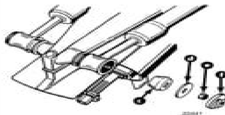
a - Anchor Pin b - Washers (2)-Large I.D. c - Rubber Bushings (4) d - Washer (2)-Small I.D. e - Locknuts (2) f - Plastic Caps (2)
