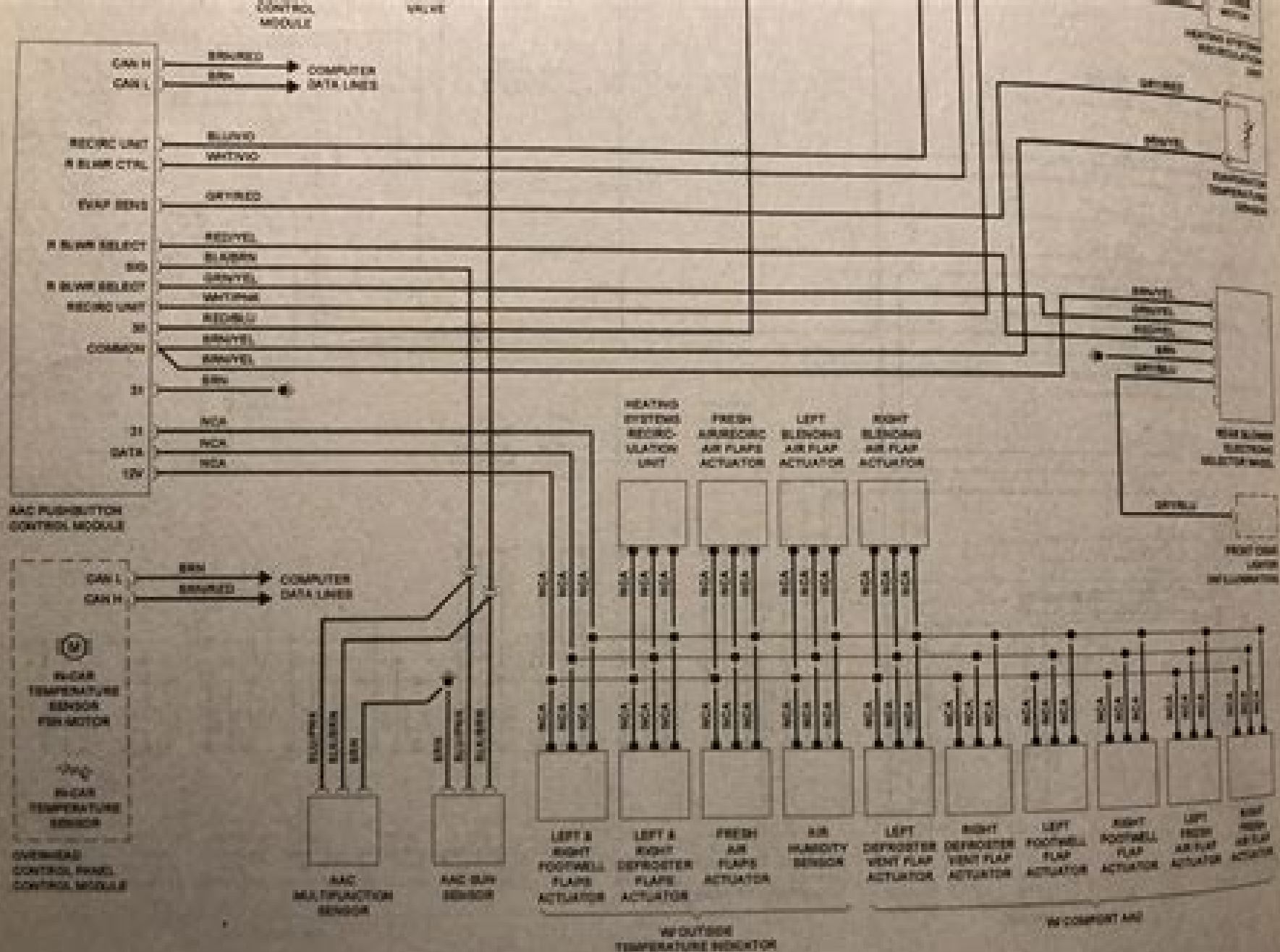
Air conditioning and engine cooling fan system - 2003 through 2005
