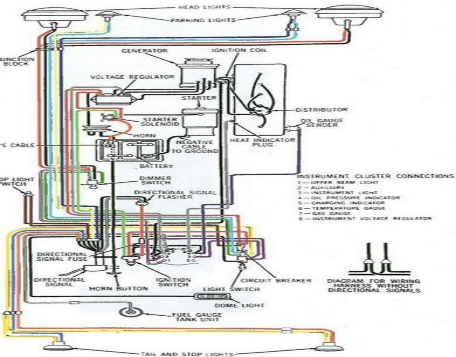
FIG. 18—WIRING DIAGRAM
