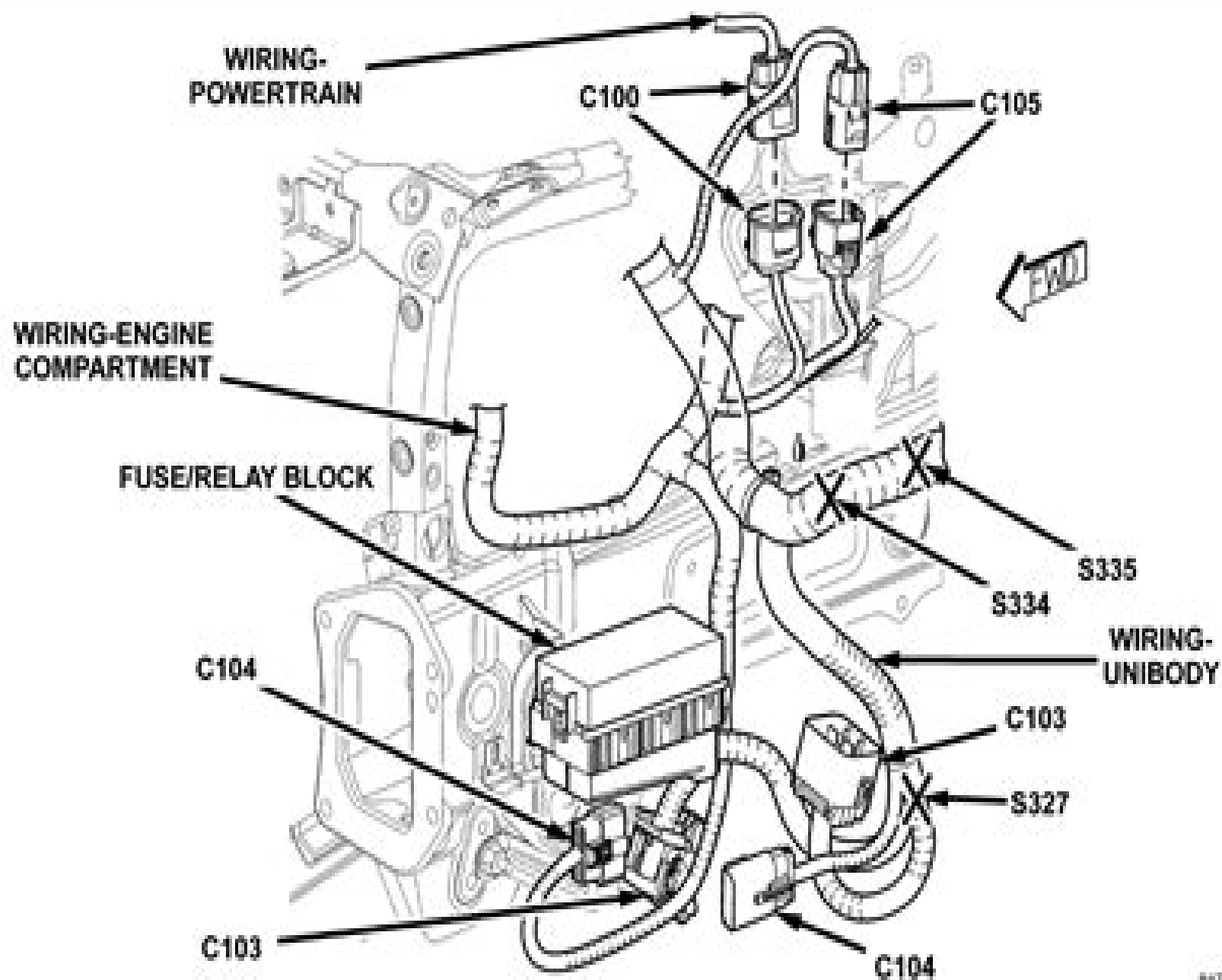
Fig. 11 FRAME RAIL - LEFT FRONT (GAS)
