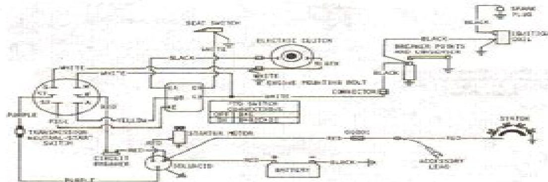
Fig. 4D101—Electrical wiring diagram for Models 108 and 111 tractors (S.N. 95001-120000).
