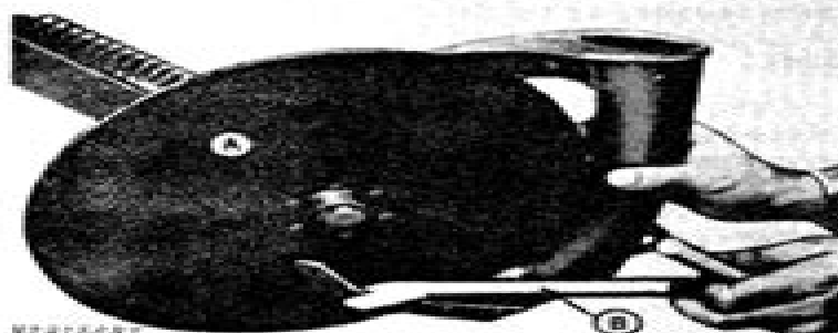
A—Toe Scraper
