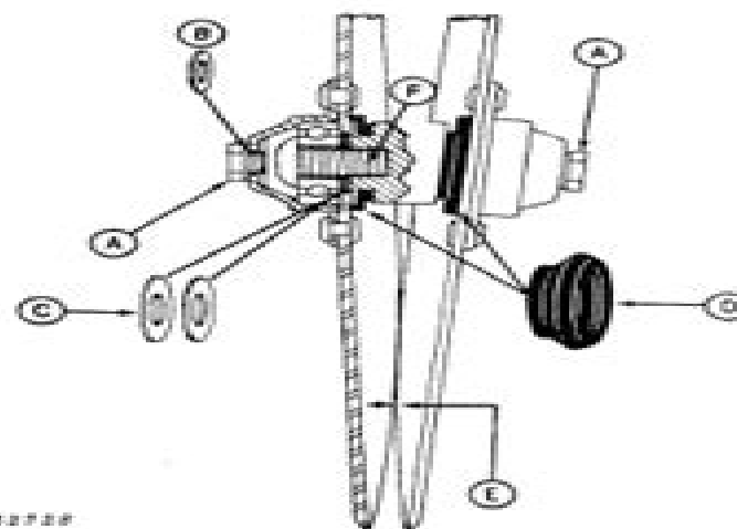
A—Bearing Plug B—Washer C—Spacer
