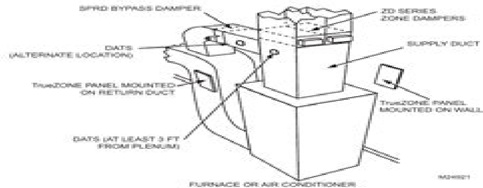
Fig. 5. Typical upflow HVAC system.
