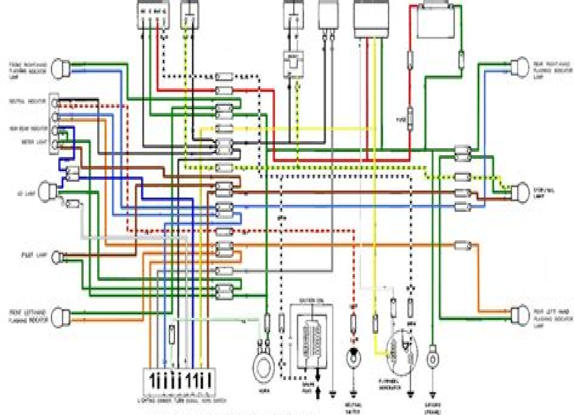
Wiring diagram - CO125B8-E/F, J and K models
