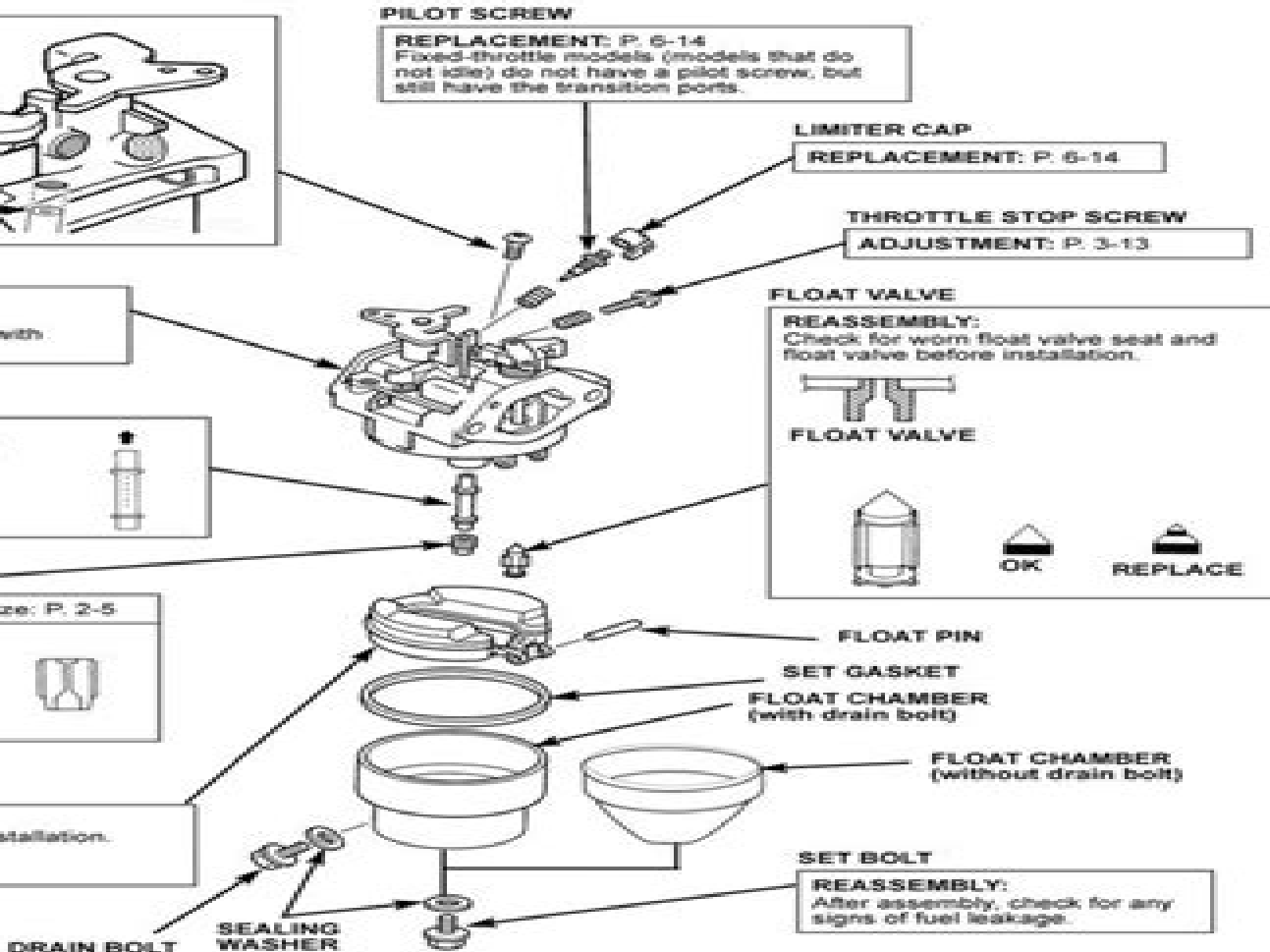
DRAIN BOLT
