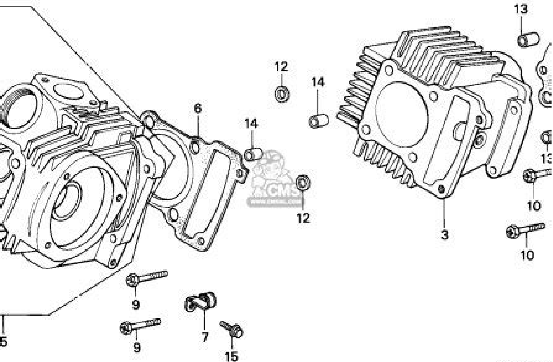
CYLINDER HEAD/CYLINDER
