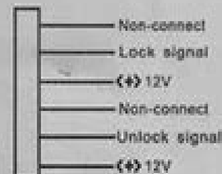
Positive trigger
