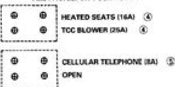
F22/1 AUXILIARY FUSE HOLDER
