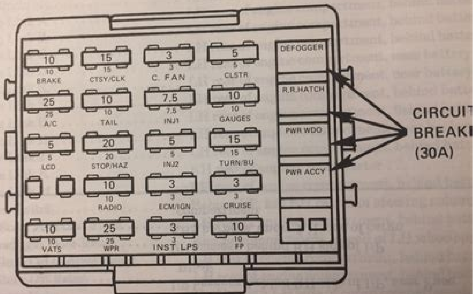
FUSE BLOCK ASSEMBLY
