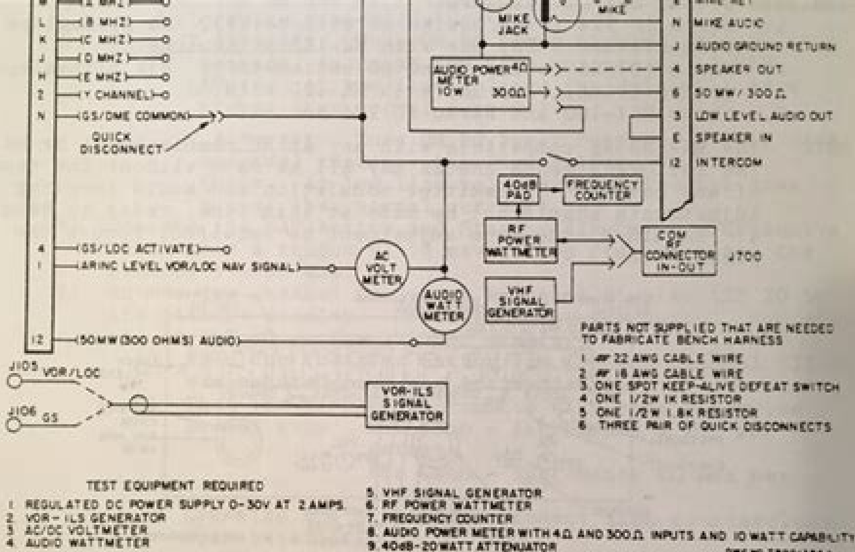
FIGURE 2-1. BENCH TEST HARNESS SET-UP
