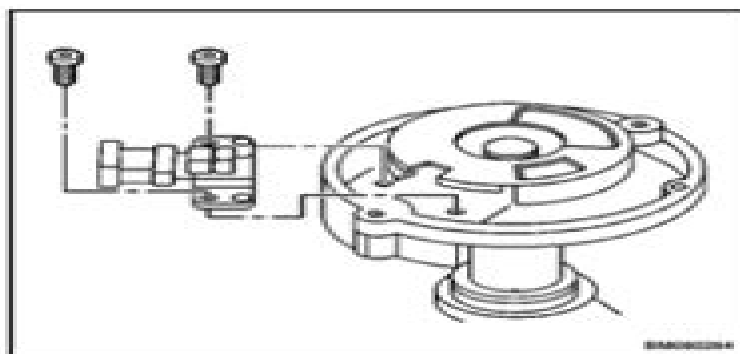
Figure 40. Camshaft Position Sensor Remove/Install
