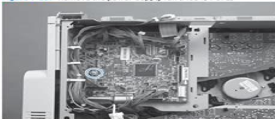
Figure 1-297 Remove the power-supply fan (M651; 1 of 2)
