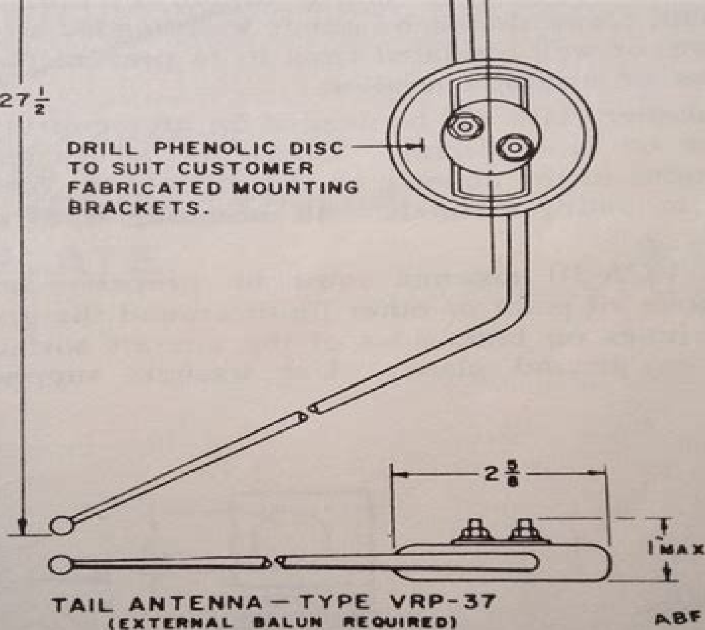
FIGURE 2-6. VRP-37
