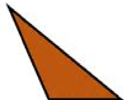
Obtuse triangle
