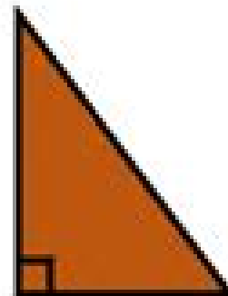
Right triangle
