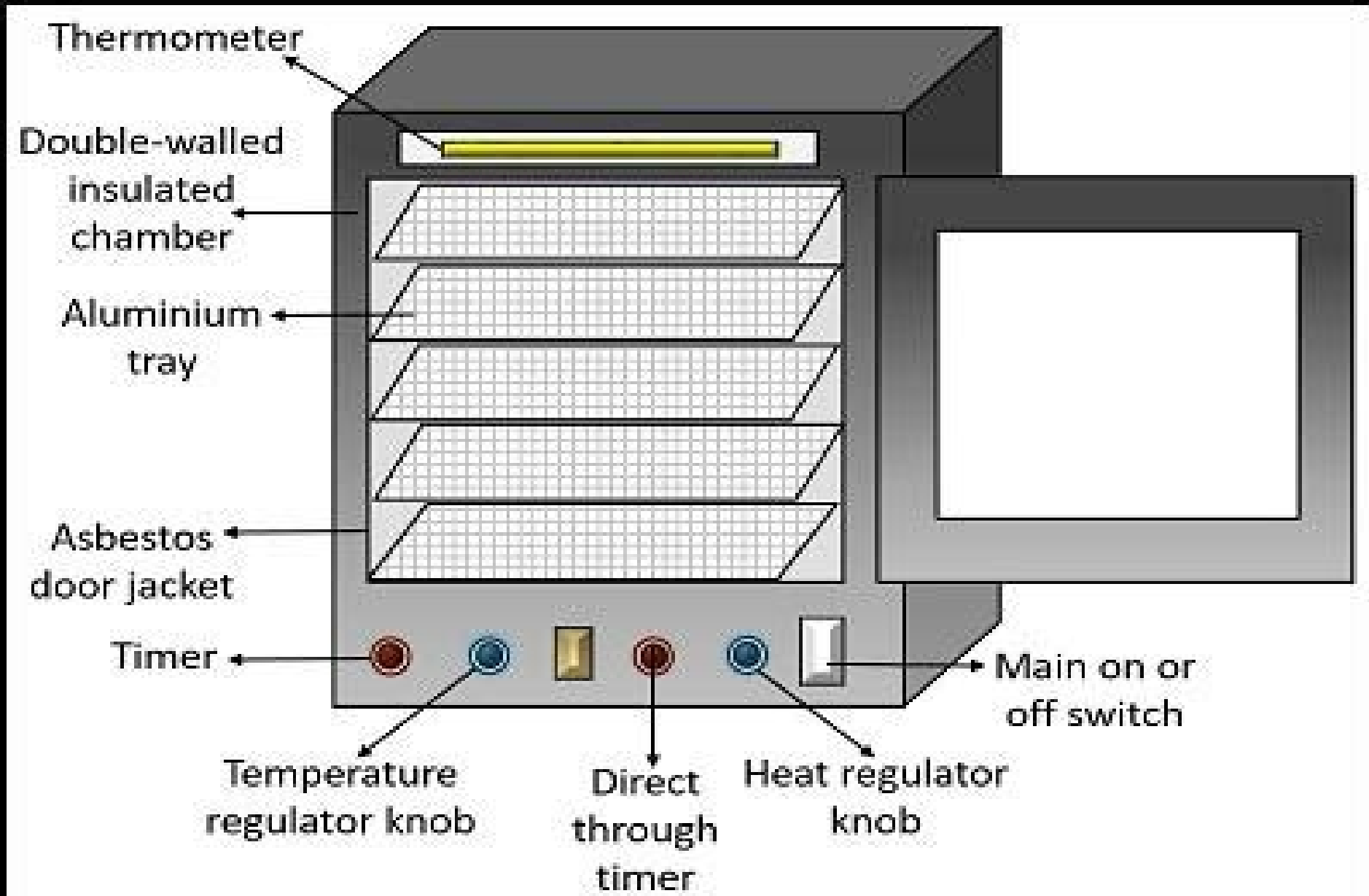
DIAGRAM OF HOT AIR OVEN
