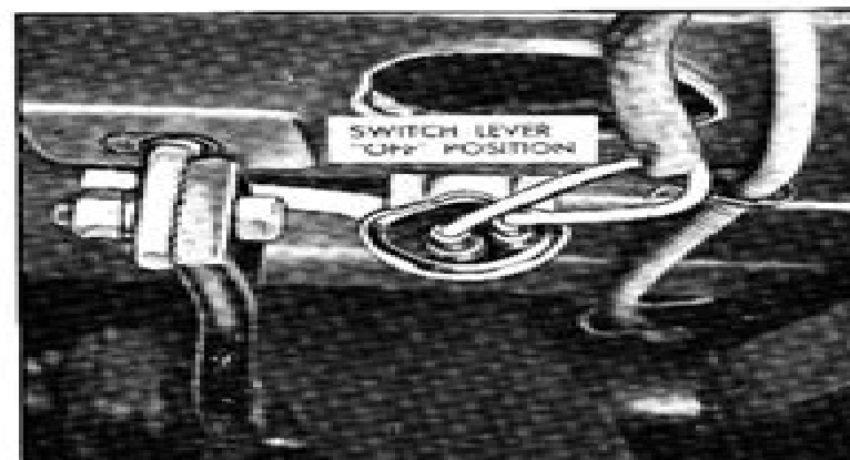
Fig. 12—Stoplight Switch Installation
