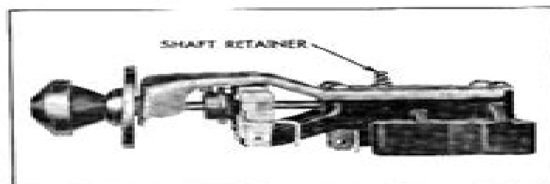
Fig. 11—Lighting Switch Shaft Retainer
