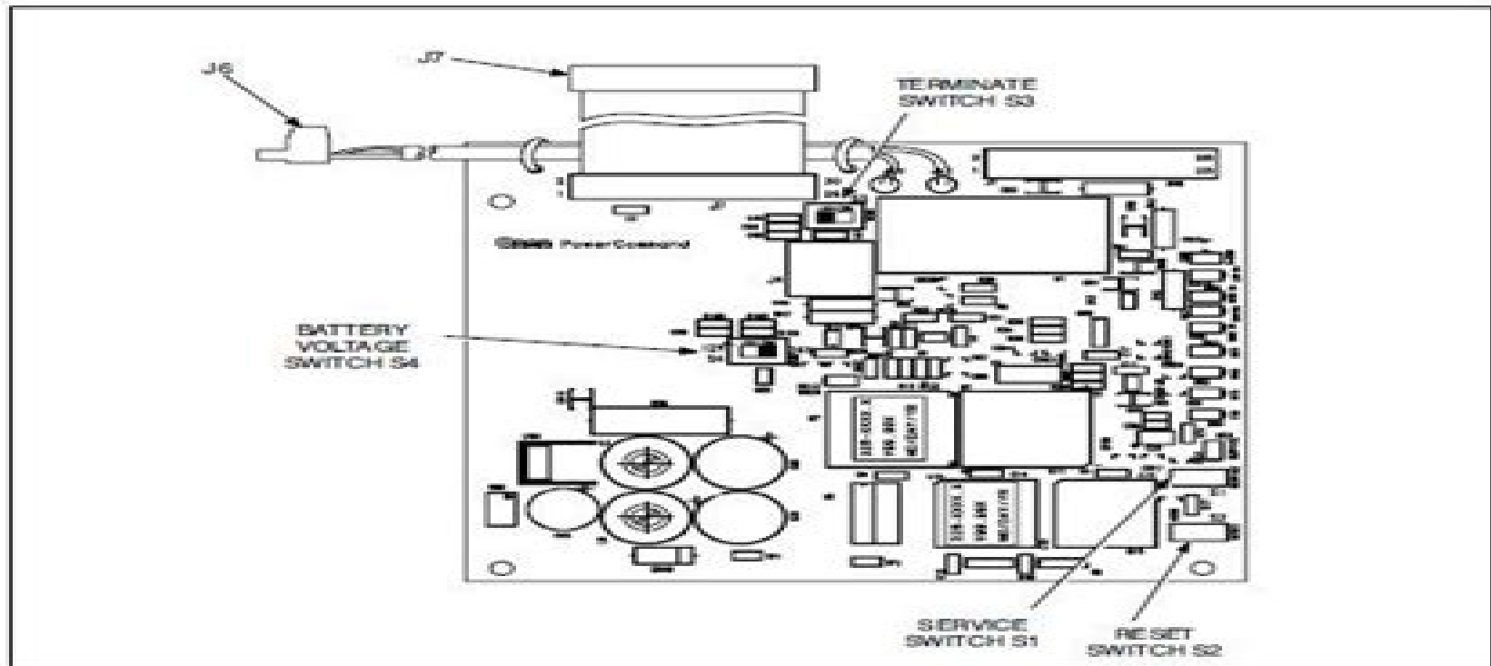
FIGURE 3-10. GENSET COMMUNICATIONS MODULE
