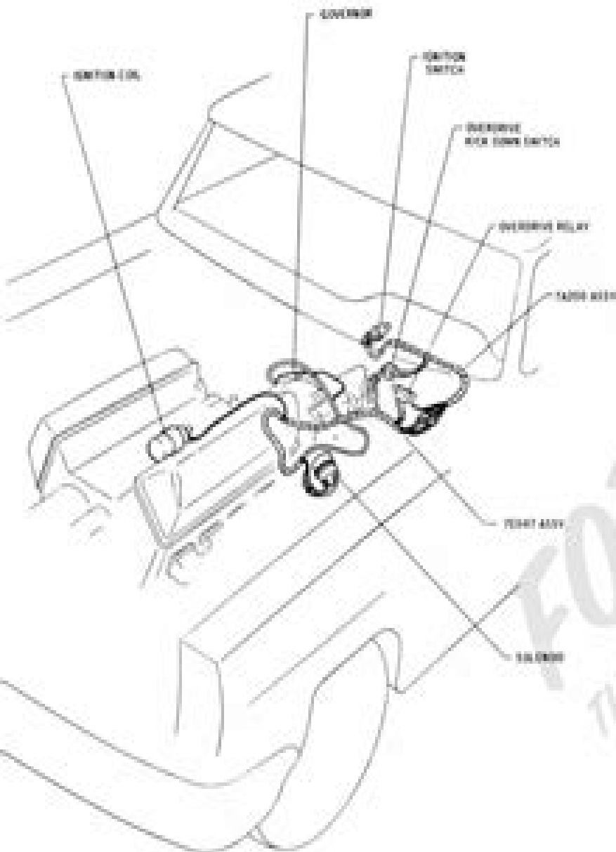
1967 FORD OVERDRIVE
