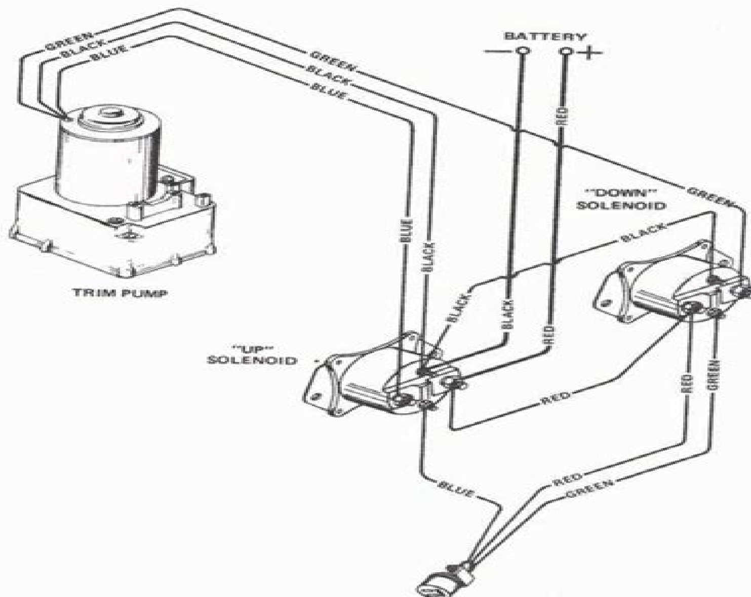
Wire Identification — Type "A" power trim/tilt system (two trim/tilt cylinders) with dual solenoids.
