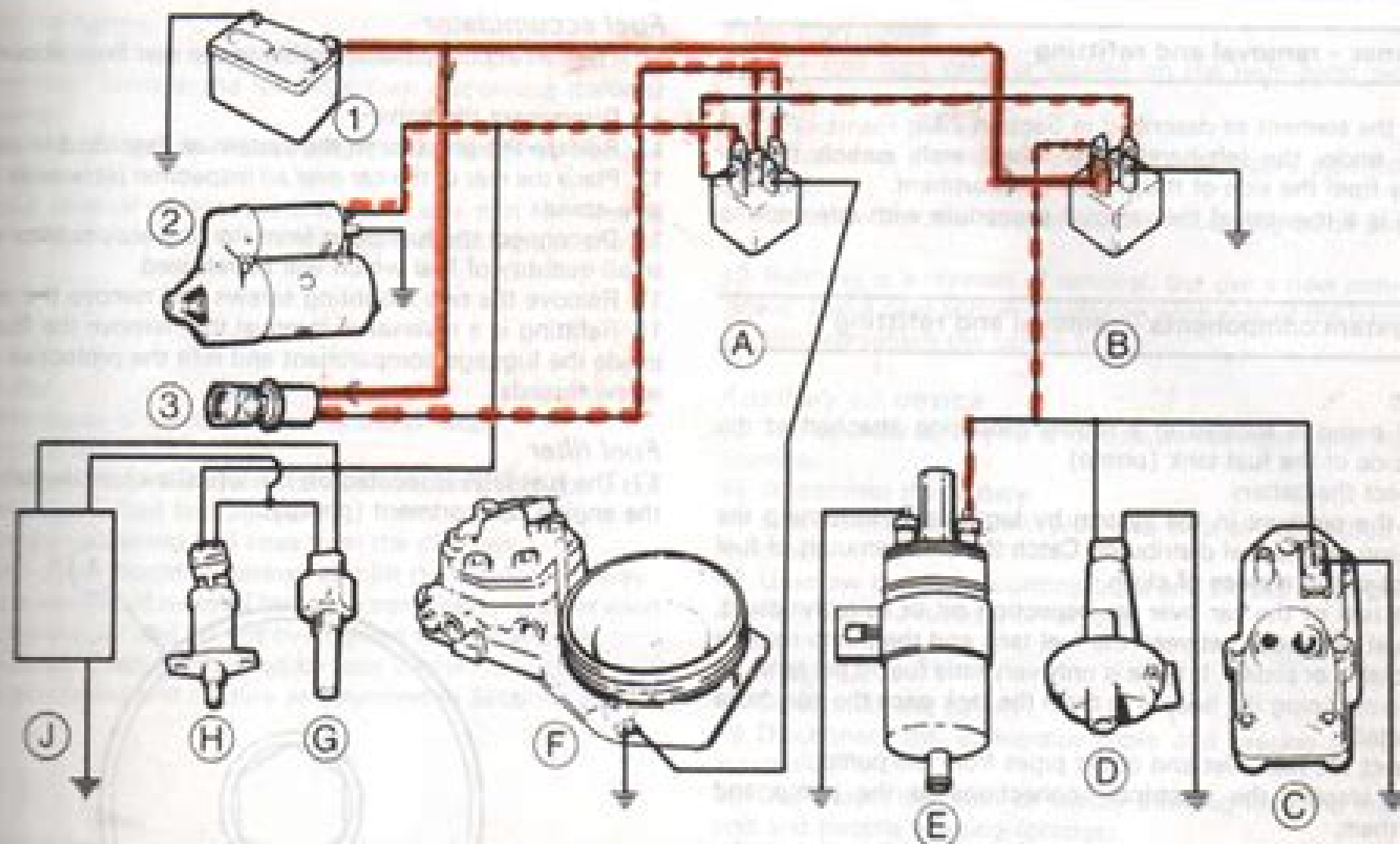
Fig. 3.33 Fuel injection system circuit diagram (Sec 22)
