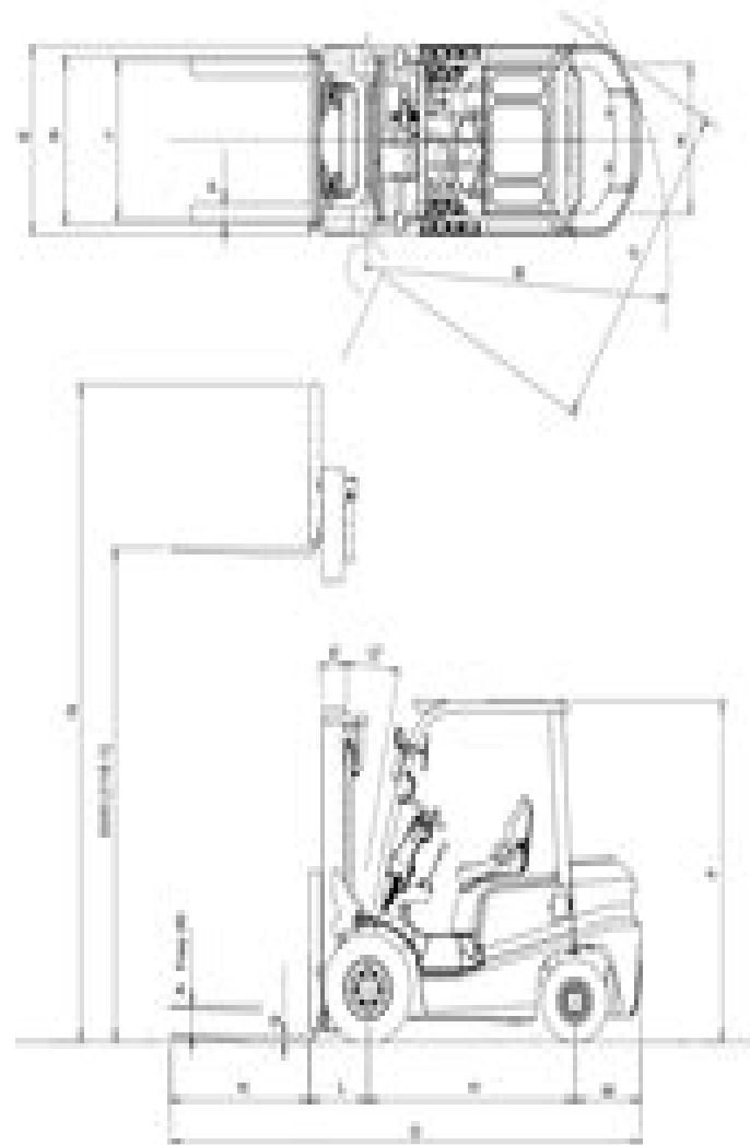
Fig. 1 Truck Dimensions
