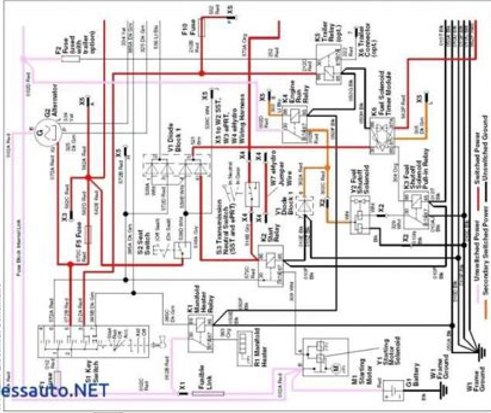
W1 Main Electrical Schematic
